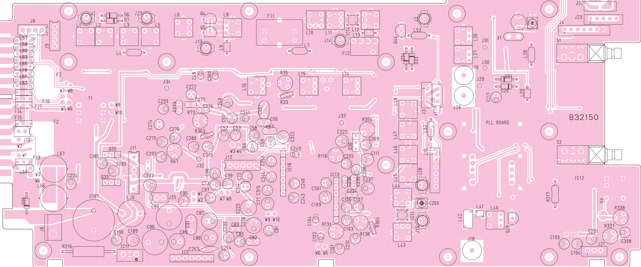
9-1 MAIN UNIT (TOP VIEW)
